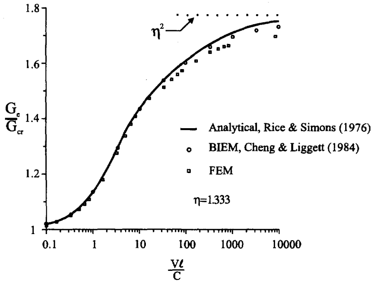
Fig. 4. Crack propagation criterion.
