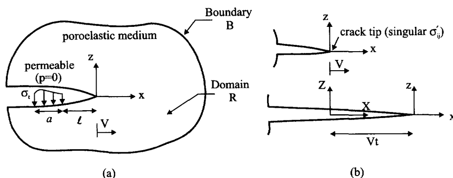
Fig. 1. Steady extension of a crack in a poroelastic medium.
