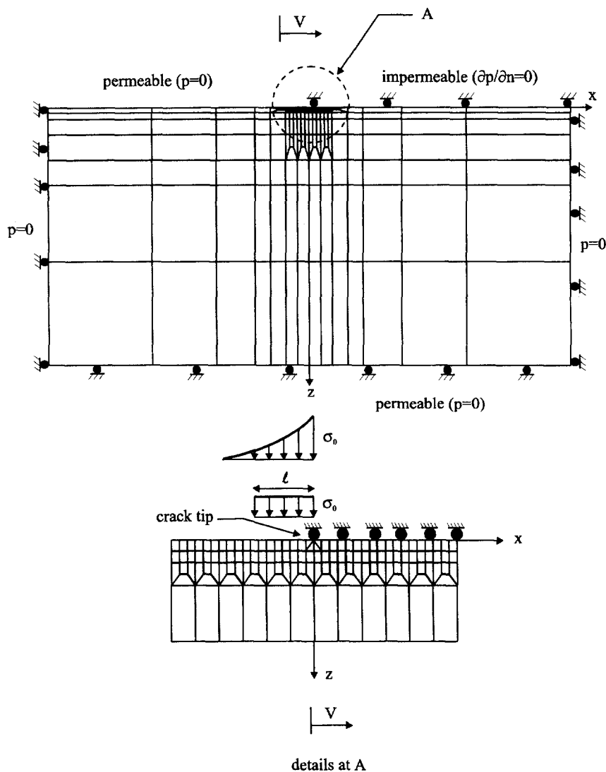
Fig. 3. Finite element discretization.
